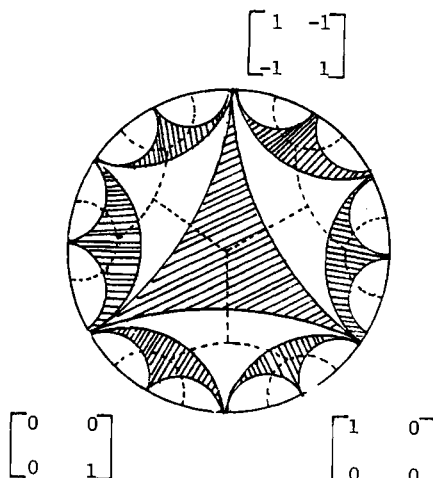
Poincaré disk with a triangulation by equilateral triangles and the dual triangulation represented by dotted lines
