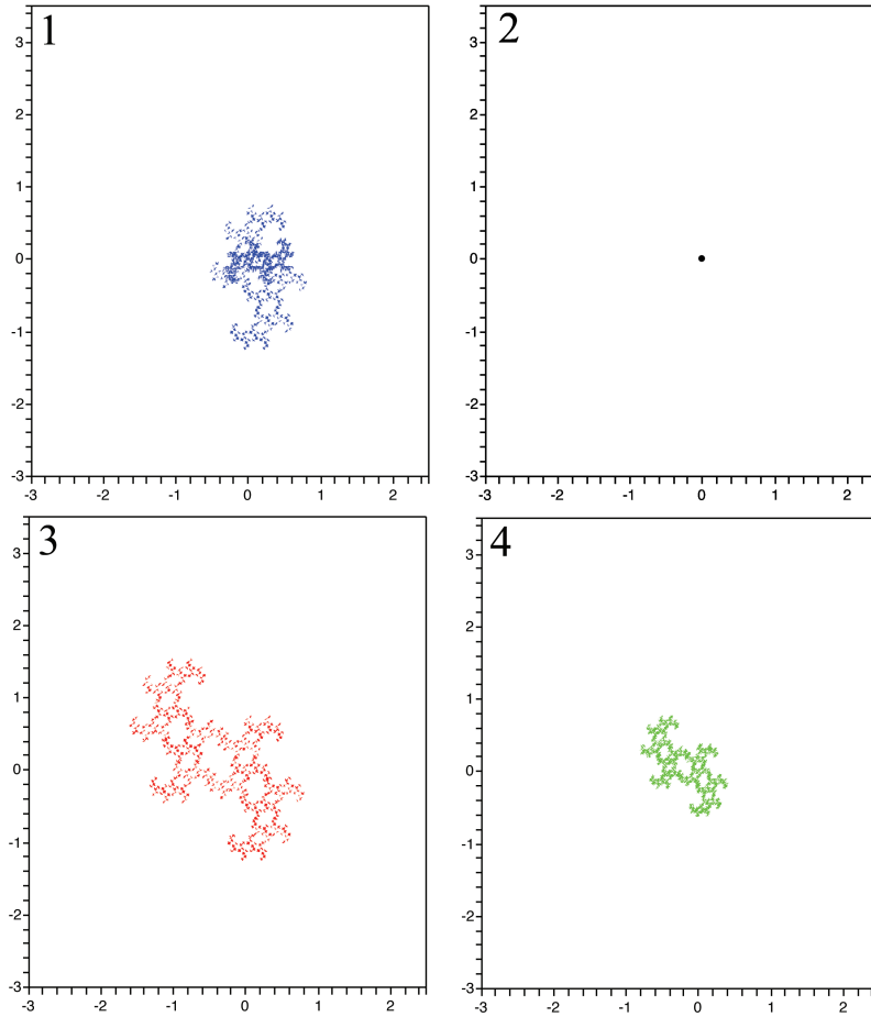
Figure 1C. The four attractors
