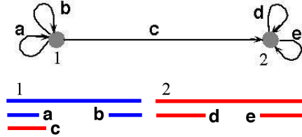
Figure 4.3A. The graph and the IFS
