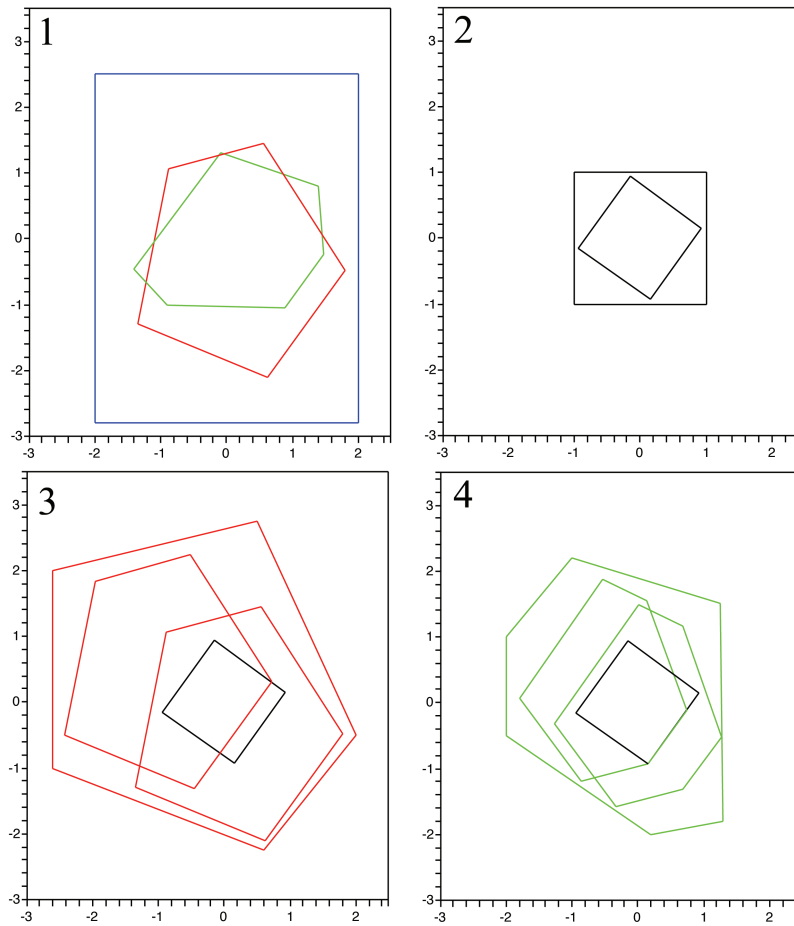
Figure 1B. Four sets mapped according to the graph
