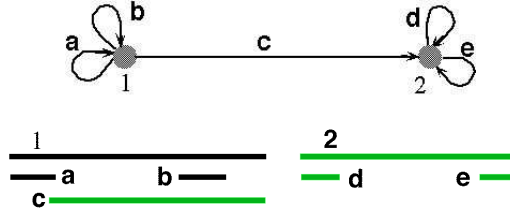
Figure 4.4A The graph and the IFS
