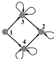
Figure 1A. A directed multigraph
